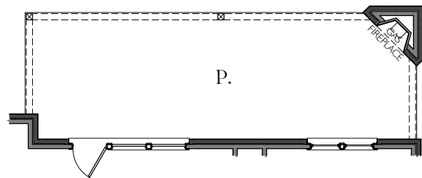
EXT. PORCH OPT. 3 w/ OPT. FP -CORNER
