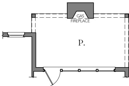
PORCH FIREPLACE OPT. 1
